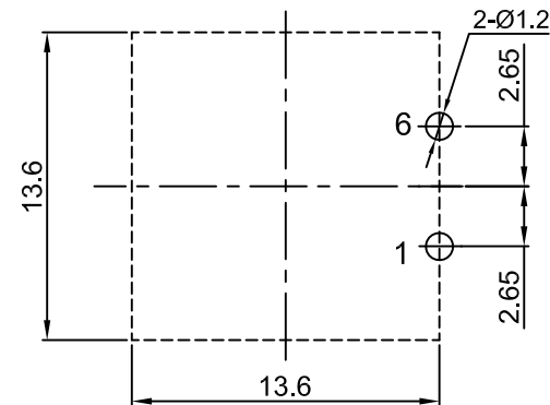
P.C.B.LAYOUT(BottomView)
