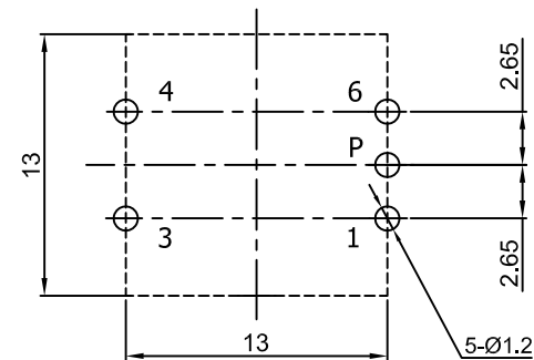
P.C.B.LAYOUT(BottomView)
