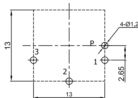
P.C.B.LAYOUT(BottomView)
